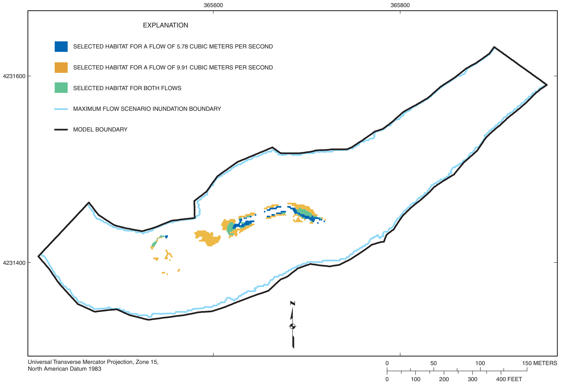
Figure 4-60. Selected habitat area distribution for habitat categories 16, 17 combined (channel catfish) at flows of 5.78 and 9.91 cubic meters per second at Marais des Cygnes River site MDC2.
